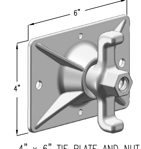
4" x 6" TIE PLATE AND NUT
