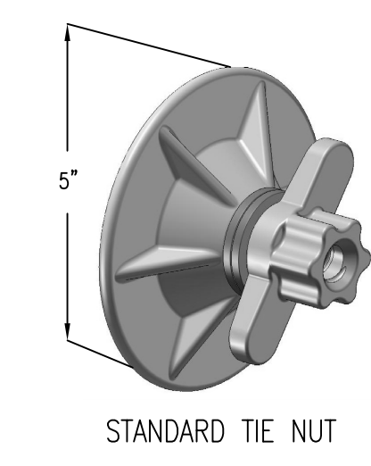
STANDARD TIE NUT
