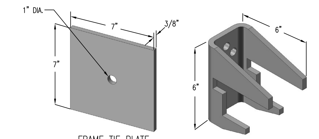
FRAME TIE PLATE TOP TIE HOLDING CLIP
