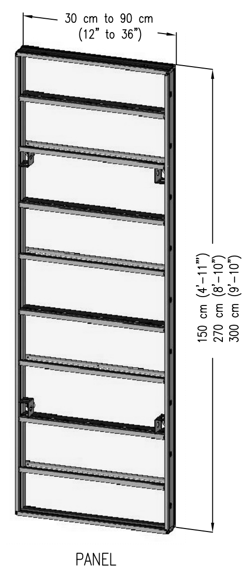
PANEL
