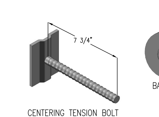
CENTERING TENSION BOLT
