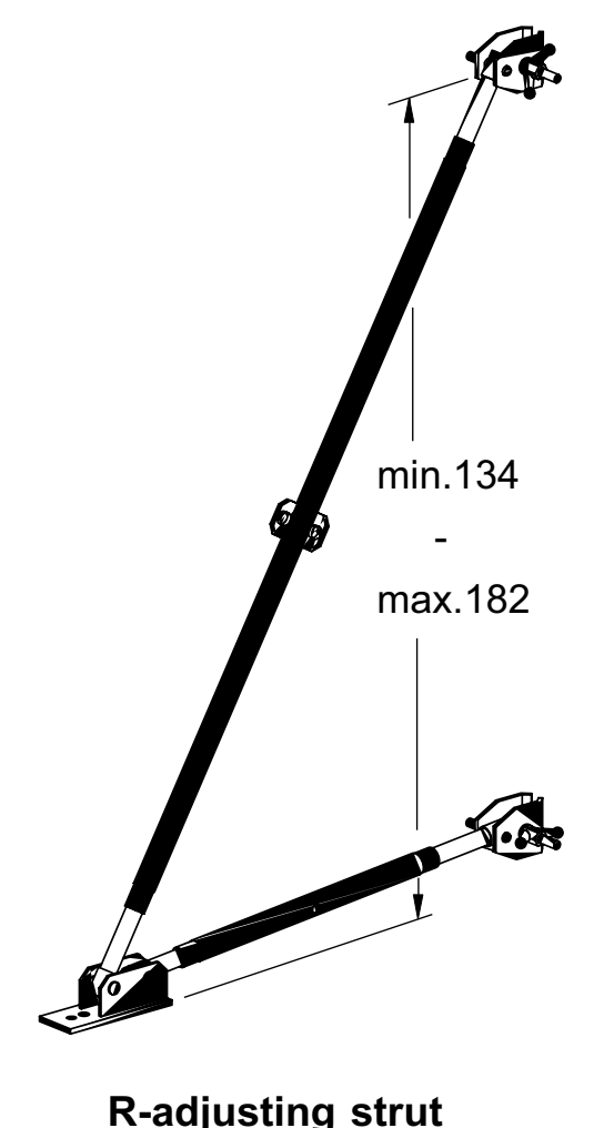
R-adjusting strut
