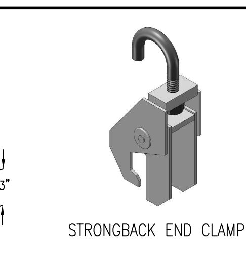
STRONGBACK CLAMP
