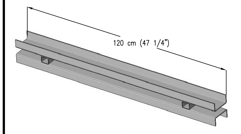
ADJUSTMENT WALER (120)
