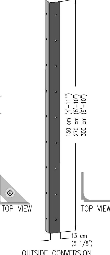
OUTSIDE CONVERSION CORNER (ALUMINUM)
