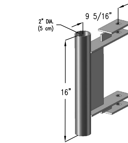
LEVELING DEVICE
