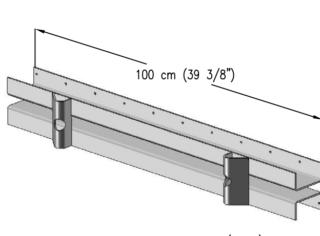
WALER MULTI-PURPOSE (100)
