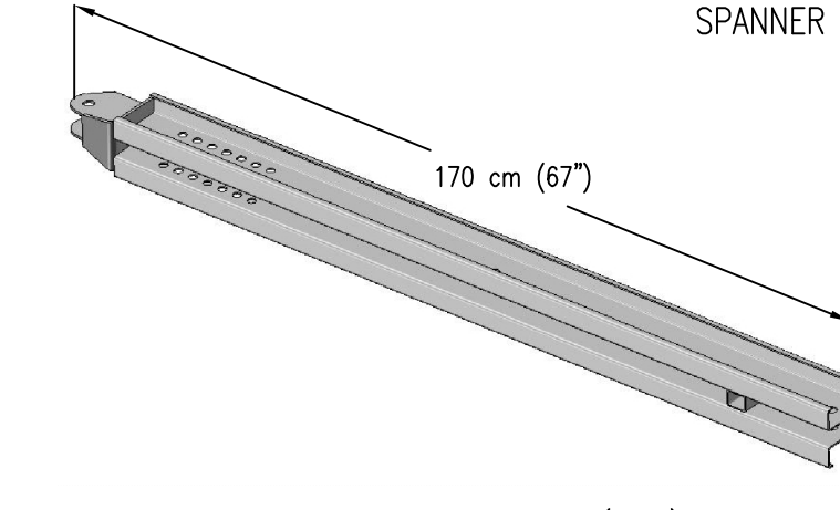
HINGED WALER (170)
