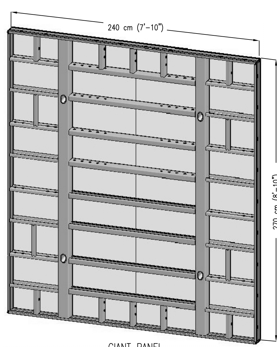
GIANT PANEL
