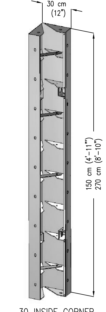
30 INSIDE CORNER RASTO Steel Faced Inside Corner RASTO Plywood faced Inside Corner
