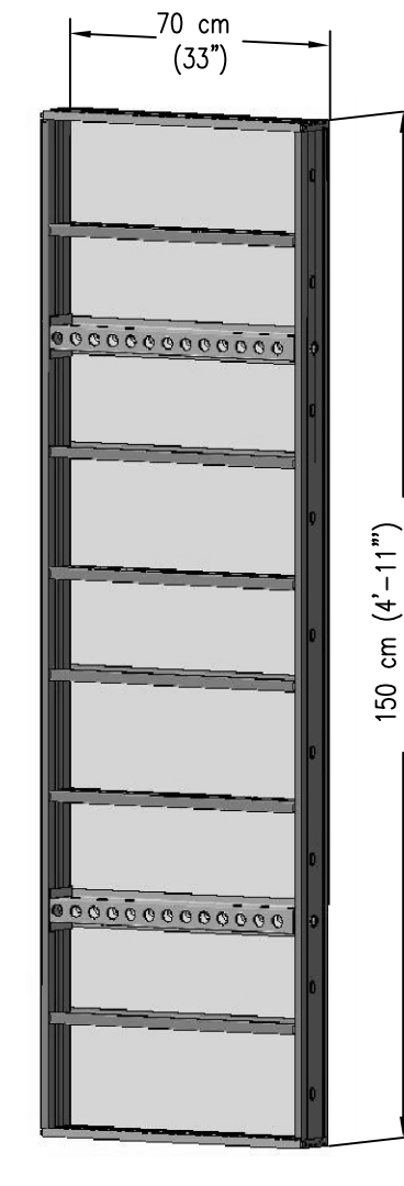
MULTI-PURPOSE PANEL
