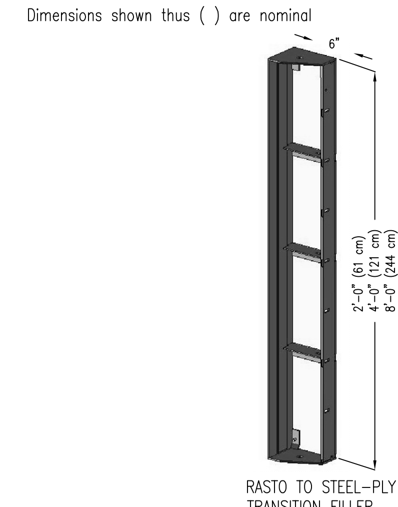
RASTO TO STEEL-PLY TRANSITION FILLER
