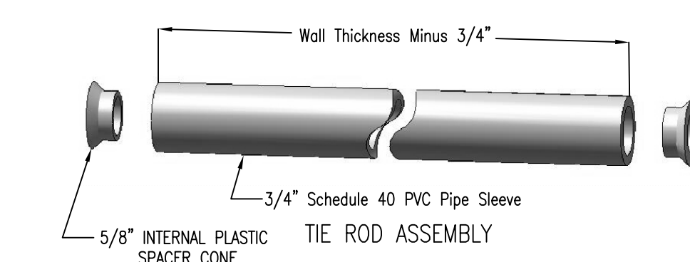
TIE ROD ASSEMBLY
