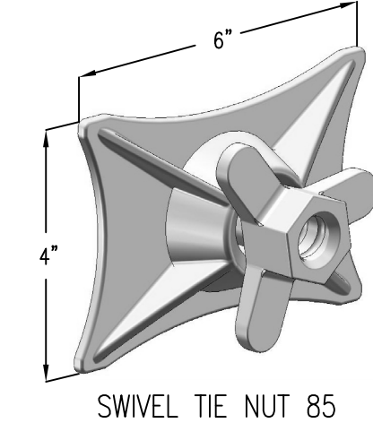
SWIVEL TIE NUT 85
