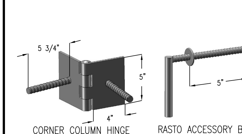
CORNER COLUMN HINGE
