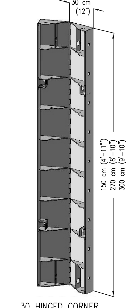
30 HINGED CORNER RASTO Steel Faced Hinged Corner RASTO Plywood faced Hinged Corner
