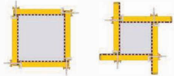
► Columns from 6" x 6" to 27" x 27" adjustable in 1" increments.
