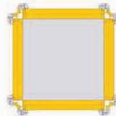
► Maximum column of 30" x 30", using universal panels with outside corners tied with fixed clamps
